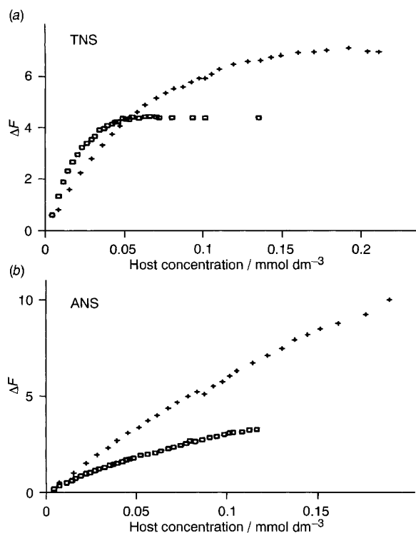
Fig. 2 Fluorescence titration with cyclodextrin-calix[4]arene hosts 1 ( \square ) and 2 ( + ) of (a) TNS ( 1.30 \times 10^{-5}\text{ mol dm}^{-3} , \lambda_{\text{ex}} = 358\text{ nm} , \lambda_{\text{em}} = 440\text{ nm} ) and (b) ANS ( 0.94 \times 10^{-5}\text{ mol dm}^{-3} , \lambda_{\text{ex}} = 354\text{ nm} , \lambda_{\text{em}} = 467\text{ nm} ), pH 7.0, 25 °C
