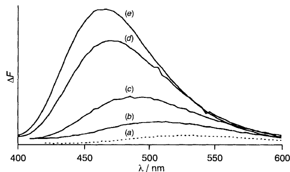
Fig. 1 Fluorescence emission spectra of (a) ANS ( 10 \times amplified), ANS with (b) \beta -cyclodextrin, (c) 3 , (d) 1 , and (e) 2 . ([ANS] = 10^{-5} mol dm -3 , \lambda_{ex} = 354 nm, \lambda_{em} = 467 nm, pH 7.0, 25 °C).
